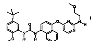
1-(5-tert-Butyl-2-methoxy-phenyl)-3-{4-[2-(2-methoxy-ethylamino)-pyrimidin-4-yloxy]-naphthalen-1-yl}-urea;
